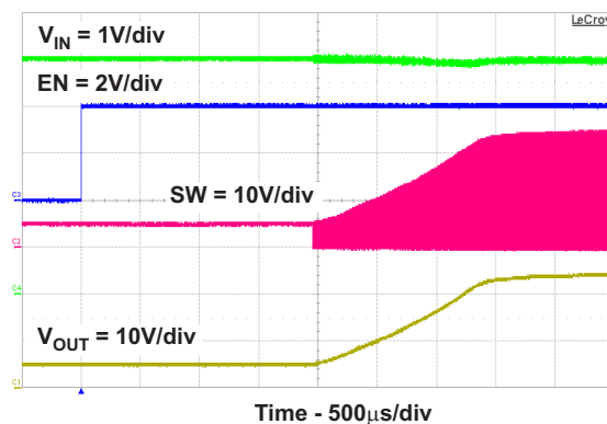
Figure 22. Start Up
