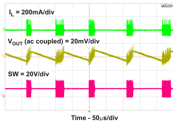
Figure 21. Pulse Skipping
